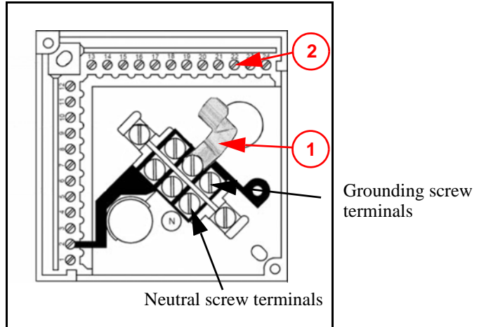
Fig 2. LFL Wiring Base
